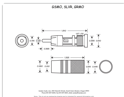
Cardas G6MO RCA plug, silver plated - DISCONTINUED
